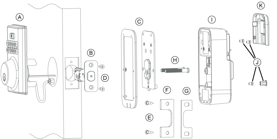
Figure 4: Smart lock installation overview
